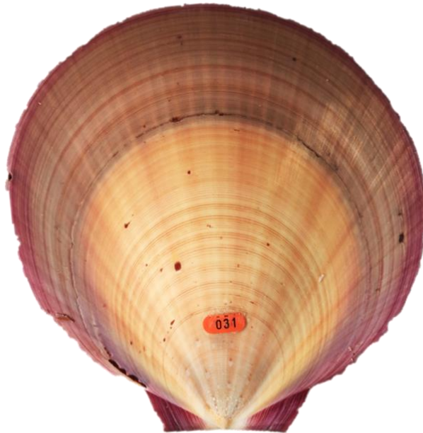
Figure 5-1. An example of a saucer scallop, Ylistrum balloti , that had been tagged and recaptured in the Abrolhos Islands. Note, growth post tagging and release is evident as rings and darker pigment.
