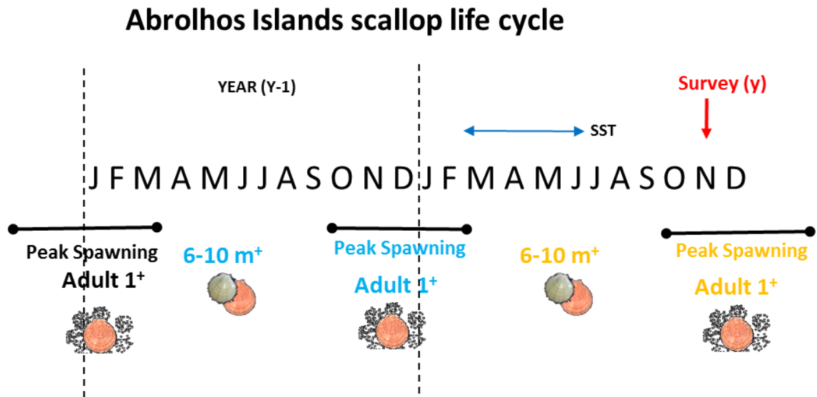
Figure 5-5. Life cycle diagram of Y. balloti along the Abrolhos Islands. Peak spawning between September and February gives rise to recruits that grow and mature over the following 12 months and enter their first spawning event by the following spring/summer (Chandrapavan et al. 2020).
